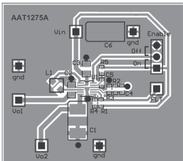
Figure 1: AAT1275A TSOPJW-12 Package Evaluation Board Top Side Layout.
