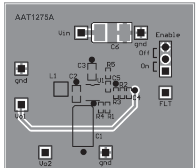
Figure 2: AAT1275A TSOPJW-12 Package Evaluation Board Bottom Side Layout.
