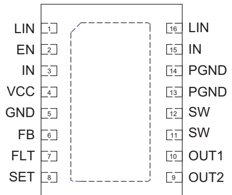
TDFN34-16 (Top View)
