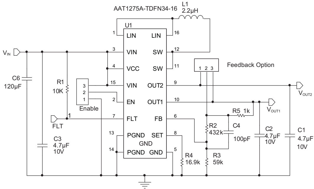
Figure 6: AAT1275A TDFN34-16 Package Evaluation Board Schematic.
