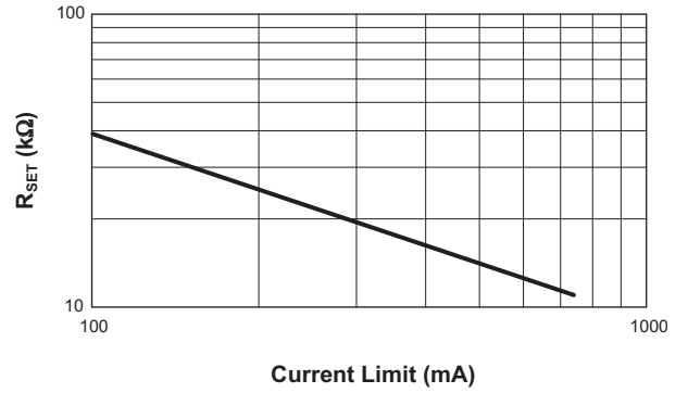
Current Limit vs. R_{SET}
